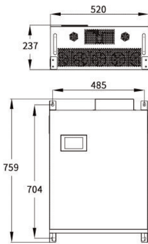
100 - 150A Wall-mounted
